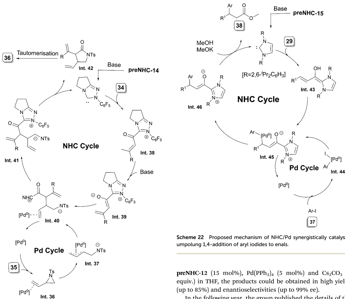
Scheme 20 Proposed mechanism of [3 + 2] annulation of vinyl enolates and vinyl aziridines via NHC/Pd synergistic catalysis.
