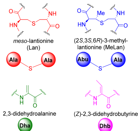
Fig. 4 Lantionine (Lan), \beta -methylantionine (MeLan), dehydroalanine (Dha) and dehydrobutyrene (Dhb) notations.
