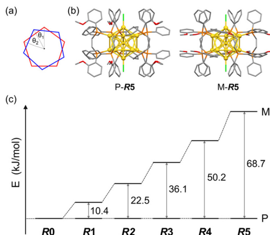
Fig. 2 (a) The torsion angles between the two equatorial \text{Au}_5 pentagons in Fig. 1c. (b) The optimized structures of P- and M- [\text{Au}_{13}(\text{R-DIPAMP})_x\text{Cl}_2]^{3+} clusters by DFT calculation. (c) The energy differences between the P- and M- \text{Au}_{13} clusters for R0–R5 .
