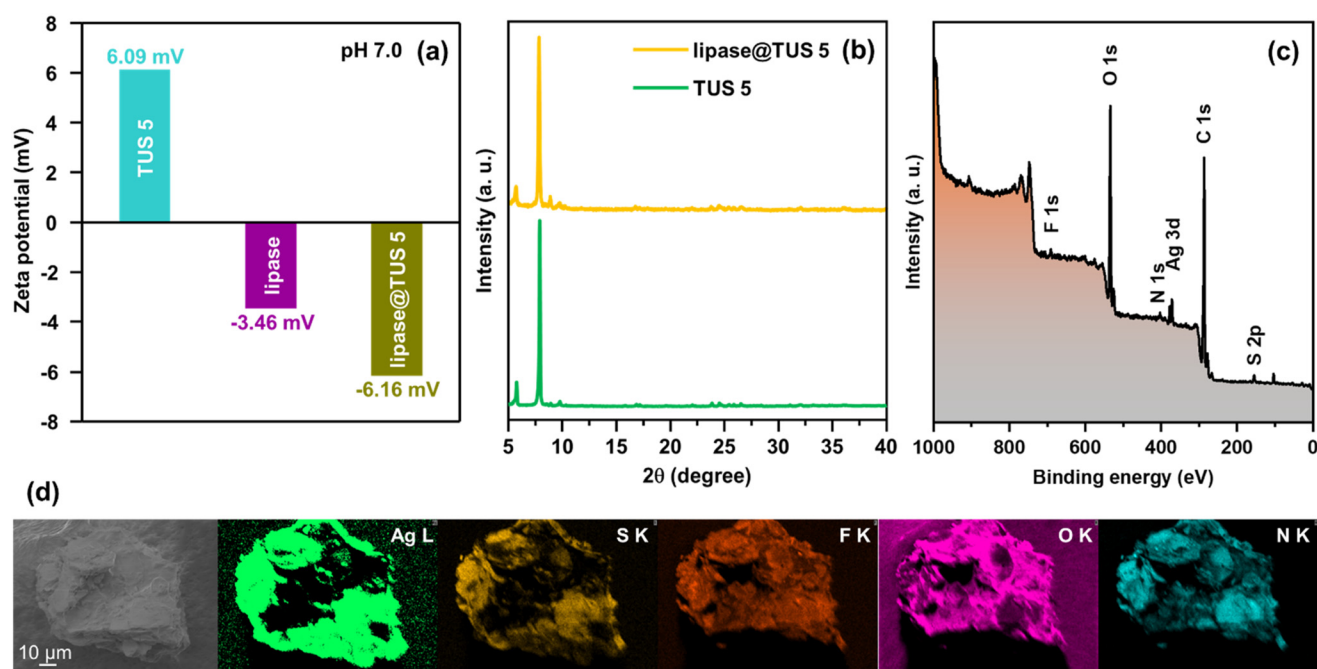
Fig. 5 (a) Zeta potential of TUS 5, lipase and lipase@TUS 5 at pH 7.0, (b) comparison between the experimental PXR patterns of lipase@TUS 5 and TUS 5, (c) wide-scan XPS spectrum of lipase@TUS 5, and (d) SEM image and the corresponding EDX elemental maps of lipase@TUS 5.
