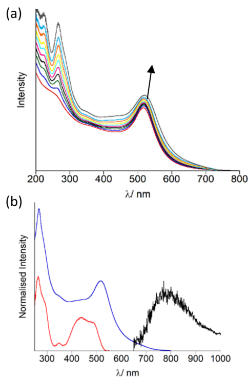
Fig. 3 Monitoring OsPhenSS coating on AuNP13 and optical spectra of isolated OsPhen-AuNP13 in water. (a) Titration of 5 \mu L quantities of 1 mM OsPhenSS (5 \mu L aliquots of 1 mM) into 4.5 nM Z-AuNP13 (4.5 nM) in aerated water and (b) isolated OsPhen-AuNP13 UV-Vis absorption spectrum: blue, excitation spectrum ( \lambda_{em} = 770 nm): red, and luminescence emission spectrum ( \lambda_{exc} = 488 nm), black.
