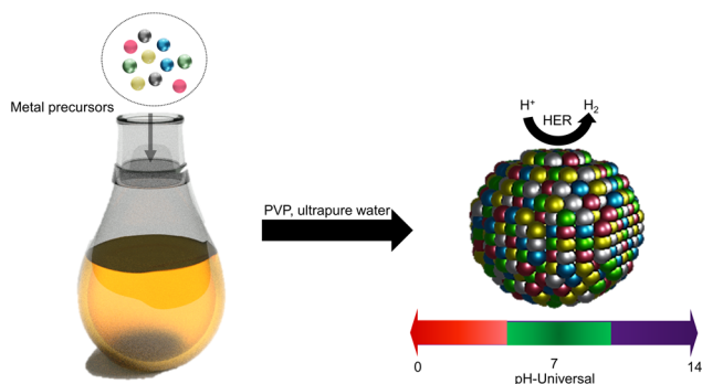
Scheme 1 The synthesis method for AuPdFeNiCo HEA nanoparticles.
