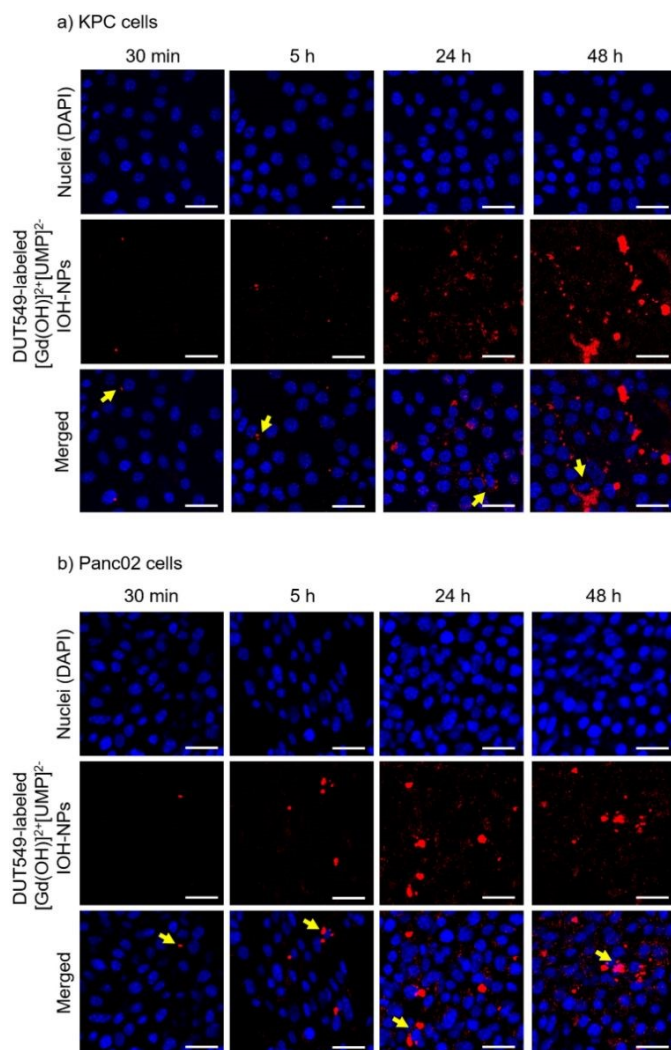
Fig. 4 Cell uptake of DUT549-labeled reference [\text{Gd}(\text{OH})]^{2+}[\text{UMP}]^{2-} IOH-NPs in a) KPC and b) Panc02 PDAC cells, monitored with confocal fluorescence microscopy over time (after 0.5, 5, 24 and 48 h of incubation at 37 °C). DUT549-labeled IOH-NPs were imaged with \lambda_{\text{ex}} = 549 \text{ nm} , \lambda_{\text{em}} = 559\text{--}650 \text{ nm} (red); DAPI staining with \lambda_{\text{ex}} = 405 \text{ nm} , \lambda_{\text{em}} = 415\text{--}479 \text{ nm} (blue). Yellow arrows on merged images point to the cells, which have taken up extraordinary high amounts of IOH-NPs. Scale bar corresponds to 25 \mu\text{m} in all images.
