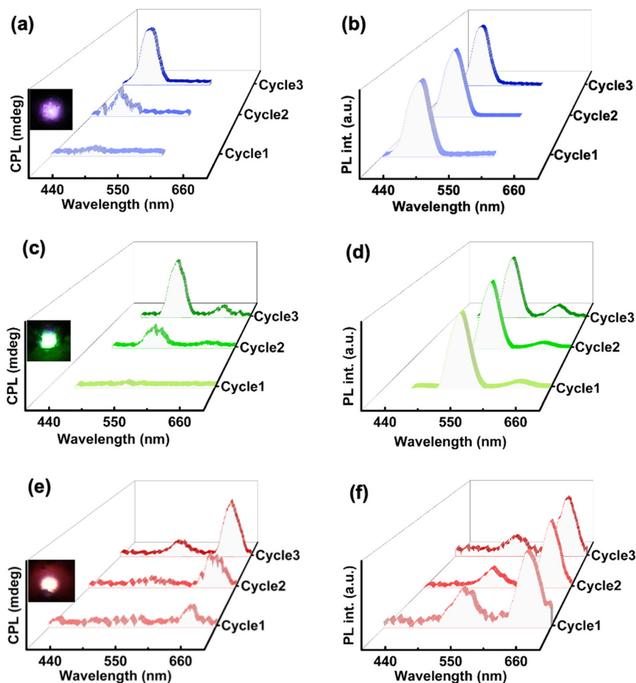
Fig. 6 (a, c and e) CPL and (b, d and f) PL spectra of UCNP-ChB nanocomposites collected from films prepared by incorporating NaYF 4 /Yb,Tm (blue traces), NaYF 4 /Yb, Mn, Ho (green traces) and NaYF 4 /Yb, Er, Mn (red traces) into the ChB. The spectra were collected for different thermal cycles after excitation using a 980 nm diode laser. Inset shows the photograph of film irradiated with the laser.
