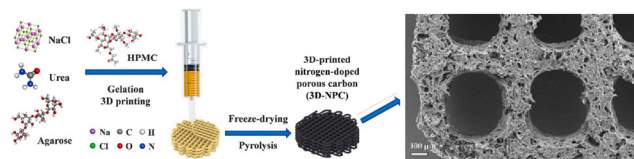
Fig. 7 Schematic for the fabrication of 3D nitrogen-doped porous carbon by DIW and the resulting morphology. 70
