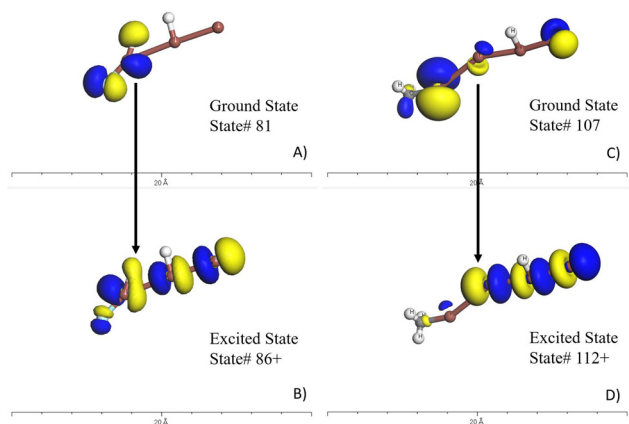
Fig. 4 TDDFT results for the FIll ( H_2FI_3 ) molecule (A and B) and C[I][I]III (C and D). Subfigure A and C illustrate the ground states local density of states. The yellow is associated with spin-up and blue is associated with spin-down electrons. Subfigure B and D are the excited states local density of states. Comparing the ground state to the excited states provide spatial information of the electron transition outlined in Table 1. It is desirable to have a high overlap of these states to avoid decoherence of the states.
