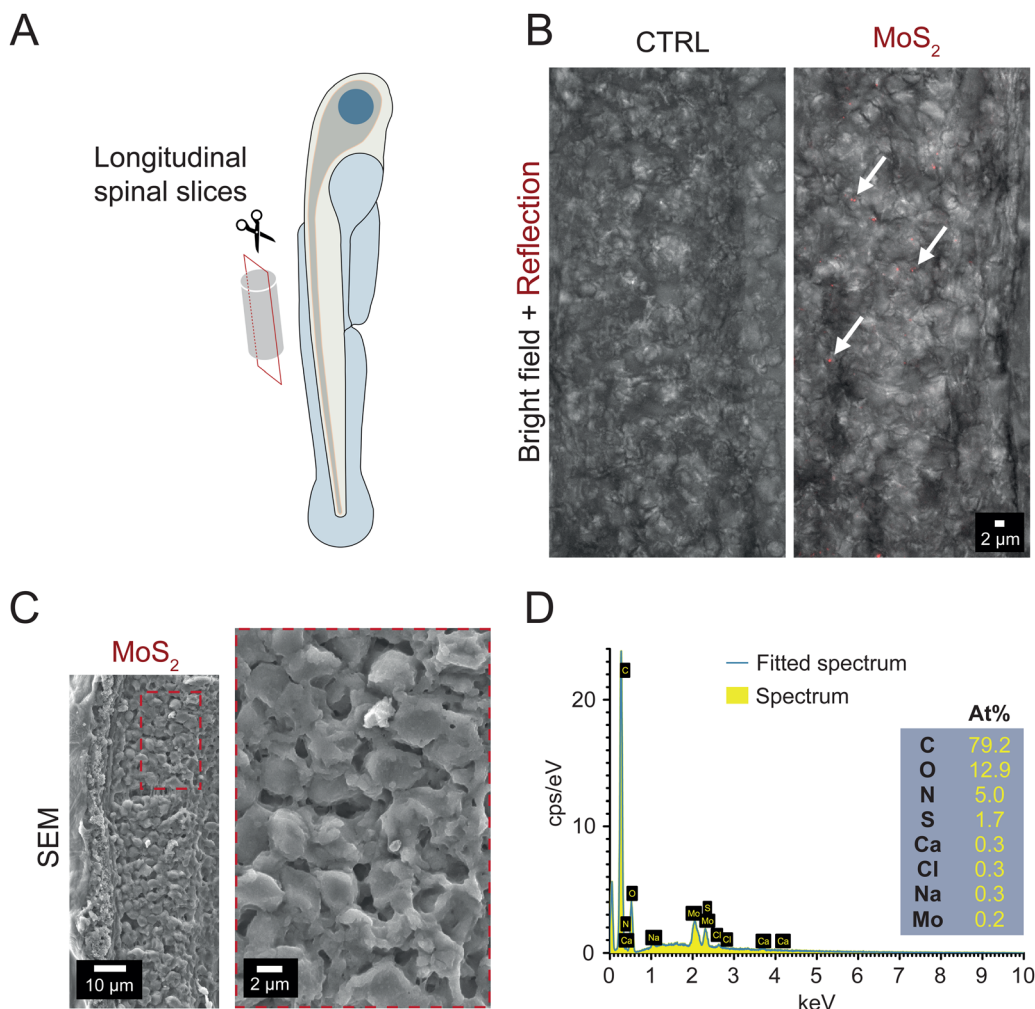
Fig. 3 After water administration, MoS 2 nanosheets are detected in the spinal cord of zebrafish. (A) Sketch of spinal cord slicing procedure to obtain longitudinal sections. (B) Z-stack reconstructions of the spinal cord of control (left) and MoS 2 exposed zebrafish (50 μg mL -1 , 2 hours; right). Images show an overlap of the bright field and reflection mode acquisitions. (C) SEM micrograph of the spinal cord obtained from larvae exposed to MoS 2 (50 μg mL -1 , 2 hours). The area in the dashed red rectangular in the left image is magnified in the right one. (D) Compositional analysis performed by EDS.
