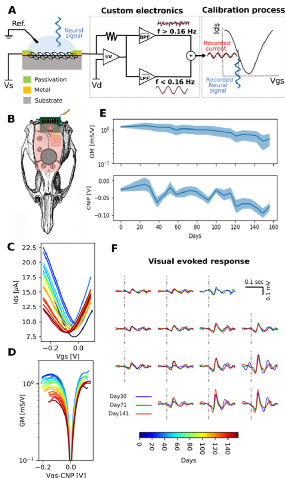
Fig. 1 Chronic stability evaluation of gSGFETs. (A) Schematic of the gSGFET recording setup and signal post-processing methodology. (B) Schematic of a rat skull depicting the location of the gSGFET array for chronic recordings. (C) and (D) Evolution of the electrical characteristics of the implanted array (C shows the transfer curve and D the transconductance). Lines represent the mean value of all transistors in the array and colors indicate implanted days. (E) Time evolution of the transconductance and CNP after implantation. Solid lines show the mean value of all transistors of the implant and shadows show the standard deviation. (F) Evolution of recorded visual evoked response at different days after implantation (averaged response for each experiment), demonstrating that the capability for recording responses remains constant over 5.5 months.
