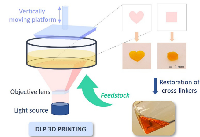
Fig. 6 Illustration of repeatable DLP 3D printing using a dynamic photocurable resin.
