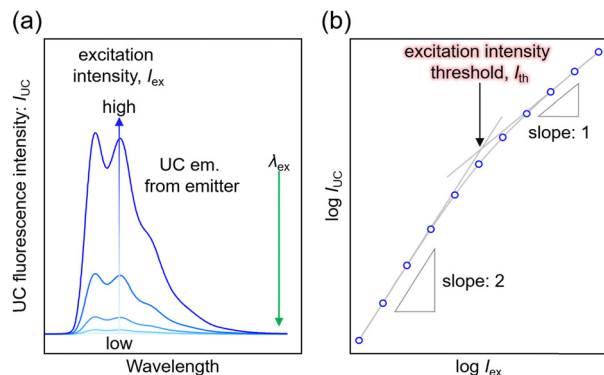
Fig. 3 (a) UC spectrum of the emitter as a function of excitation intensity and (b) log-log plot of UC intensity versus excitation intensity in a solution system consisting of sensitizer and emitter (Sen/Em). Note that these data were not obtained experimentally.
