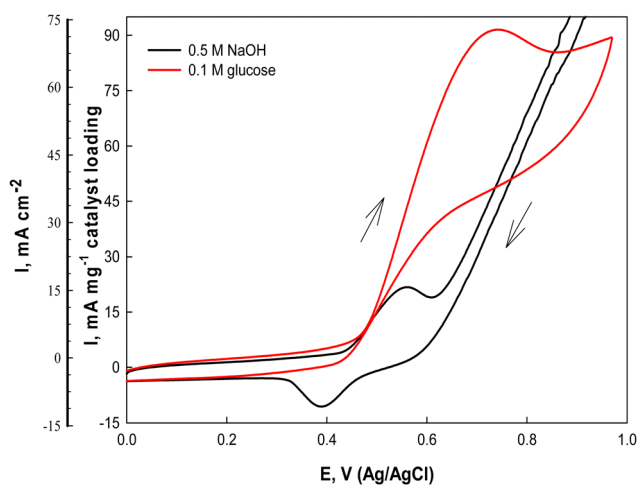
Fig. 7 Cyclic voltammograms of the Ni(II)-SB/C electrode in 0.5 M NaOH and in the presence of 0.1 M glucose at 0.02 \text{ V s}^{-1} .
