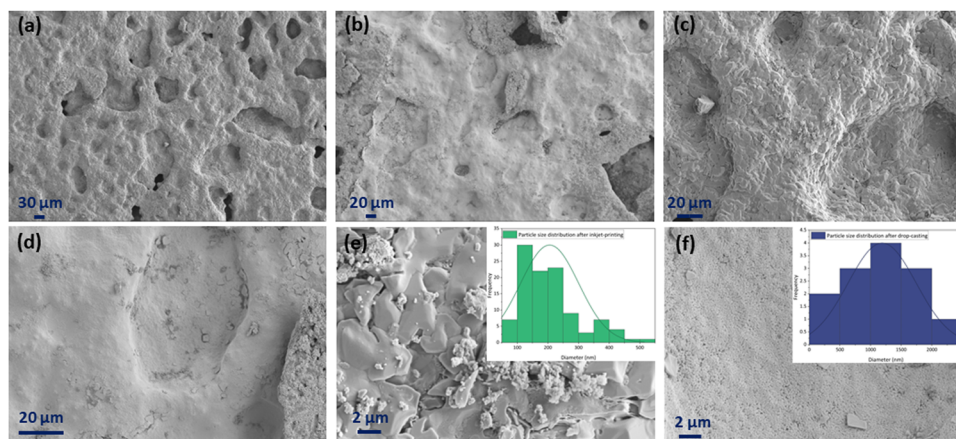
Fig. 10 Surface SEM images of (a), (c) and (e) 100-layer and (b), (d) and (f) drop-cast porous NLK–GDC symmetric cells in 185× (a and b), 687× (c and d), and 4.15k× (e and f) magnifications. The insets of (e) and (f) figures are the particle size distributions of CuFe 2 O 4 particles on the surface of the inkjet-printed and drop-cast samples, respectively, analyzed using ImageJ software.
