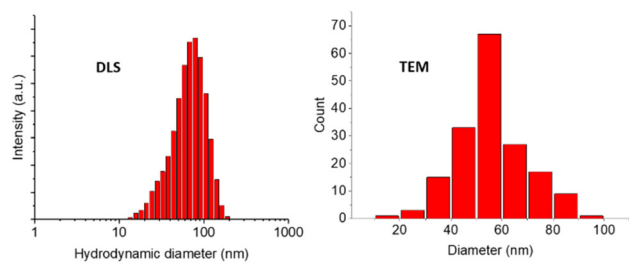
Fig. 2 GMA-EGDMA nanogel at 31% monomer conversion was analyzed by DLS and TEM displaying unimodal distribution for both techniques.
