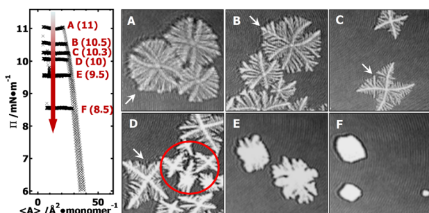
Fig. 2 BAM images [ 1.6 \times 1.6 mm 2 ] for X_{PtBA} = 0.14 PCL/PtBA blends at 22.5 °C obtained during isobaric experiments at \Pi = (A) 11, (B) 10.5; (C) 10.3, (D) 10, (E) 9.5, and (F) 8.5 mN m -1 . BAM images were taken at \langle A \rangle \sim 8 – 10 Å 2 per monomer and also represent different crystallization time (time/hour): (A) 0.3, (B) 0.7; (C) 1.5, (D) 2.7, (E) 6.8, and (F) 7.6.
