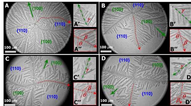
Fig. 3 OM images of a single layer LS-film transferred at \langle A \rangle \sim 5 Å 2 per monomer for a X_{PtBA} \sim 0.14 PCL/PtBA blend crystallized \Pi = (A) 11, (B) 10.5; (C) 10.3, and (D) 10 mN m -1 , respectively. The “winning” branches in \{100\} sectors and the tips of main dendritic trunks are shown in (A'–D') and (A''–D''), respectively.
