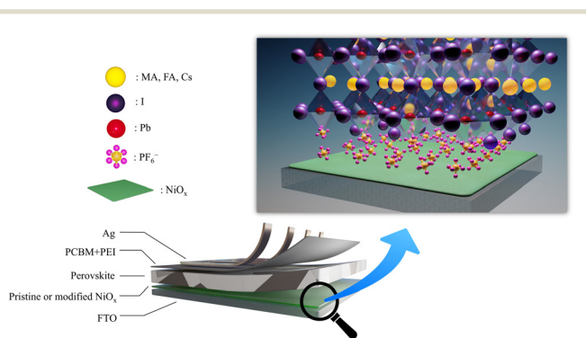
Fig. 1 Device architecture of PSCs with the enlarged illustration of the salt-modified \text{NiO}_x /perovskite interface.
