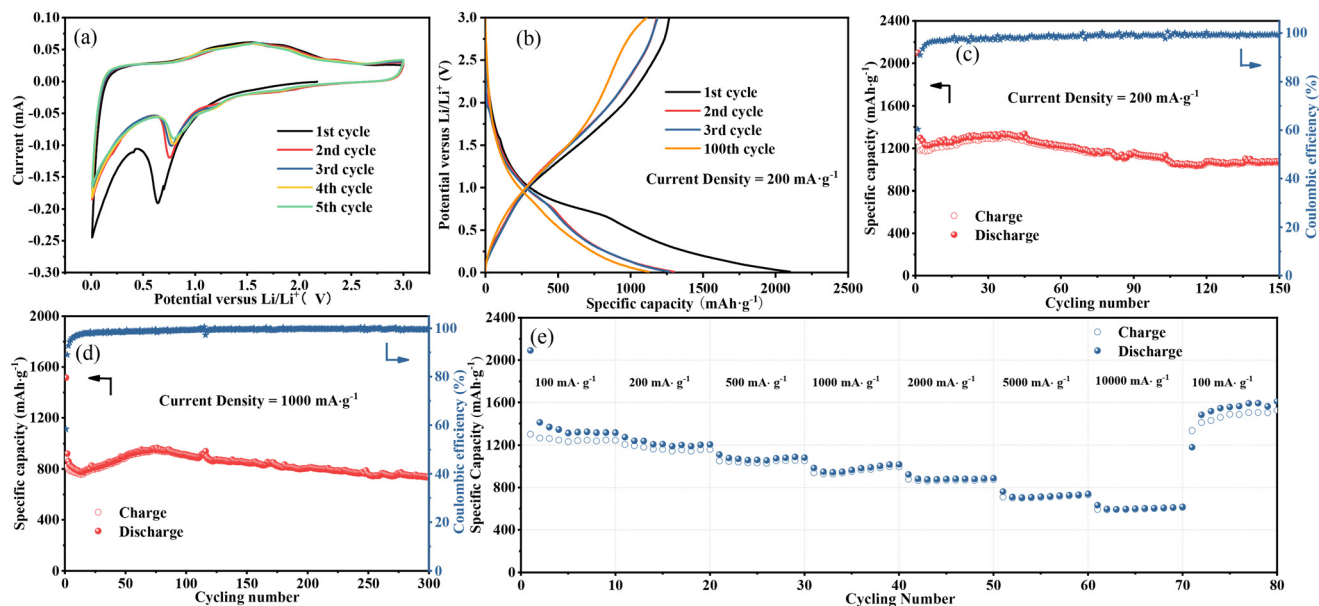
Fig. 4 The CV curves for the initial 5 cycles (a), and charge and discharge voltage profile (b) of the Fe 3 O 4 QDs@C/RGO composite. Cycling performance under a low current density of 200 mA g -1 (c), long-term lithium-ion storage capability under a current density of 1000 mA g -1 (d), and rate capability (e) of the Fe 3 O 4 QDs@C/RGO composite.
