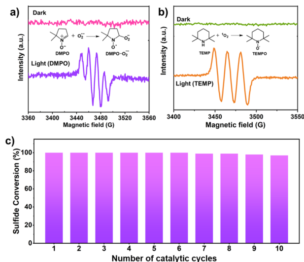
Fig. 5 EPR detection of in situ generated (a) O 2 •- with DMPO, (b) 1 O 2 with TEMP over HEP-FL, and (c) recyclability studies of HEP-FL.
