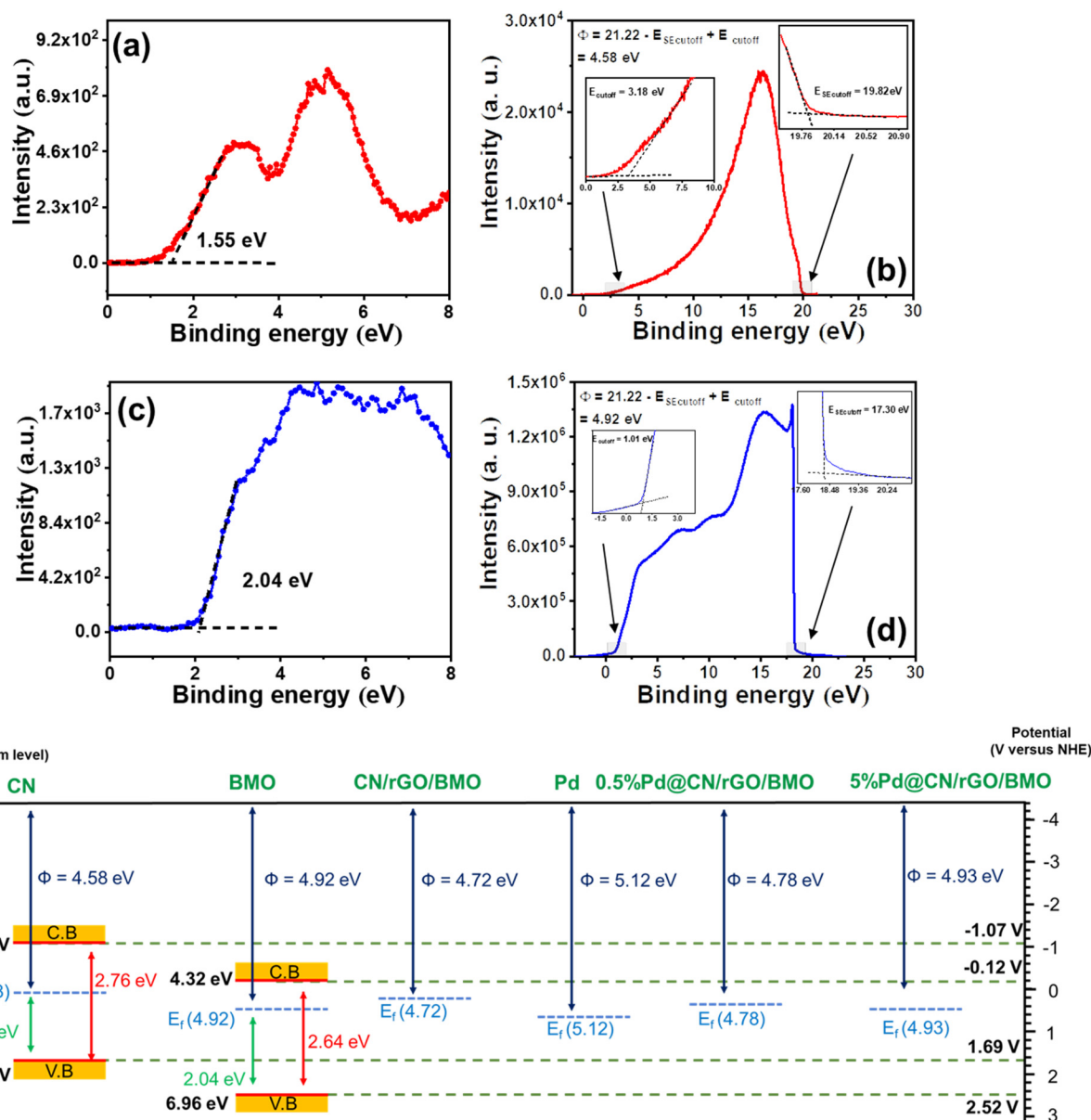
Fig. 6 (a) VB-XPS spectrum for CN, (b) UPS spectrum for CN, (c) VB-XPS spectrum for BMO, and (d) UPS spectrum for BMO and (e) (a)calculated band-structures for CN, BMO, CN/rGO/BMO(2 : 1), 0.5%Pd@CN/rGO/BMO(2 : 1), and 5%Pd@CN/rGO/BMO(2 : 1).
