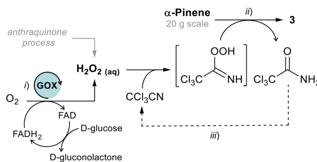
Scheme 3 Reaction conditions: for steps (i) and (ii) see Table 1; (iii) 0.8 eq. \text{P}_4\text{O}_{10} , refluxing xylene.
