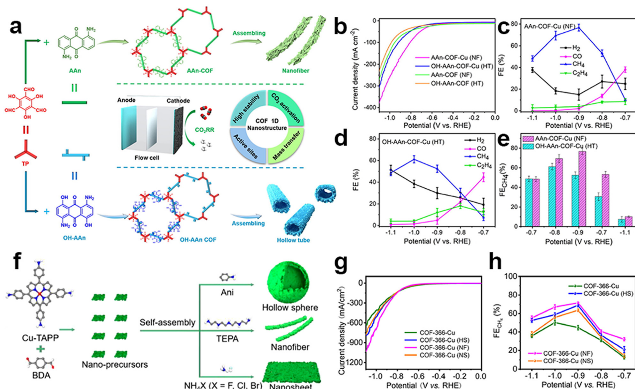
Fig. 12 Schematic illustration of super-structured COFs and their performance. (a) The schematic representation of anthraquinone COF-based nanofibers and hollow tubes in the electrocatalytic e\text{CO}_2\text{RR} ; (b) LSV curves of AAn-COF-Cu (NF), OH-AAn-COF-Cu (HT), AAn-COF (NF) and OH-AAn-COF(HT); (c–e) FE of AAn-COF-Cu(NF) and OH-AAn-COF-Cu(HT). 133 (f) The schematic representation of porphyrin COF-based nanostructures; (g) LSV curves and (h) \text{FE}_{\text{CO}} values of COF-366-Cu, COF-366-Cu(HS), COF-366-Cu(NF) and COF-366-Cu(NS). 134
