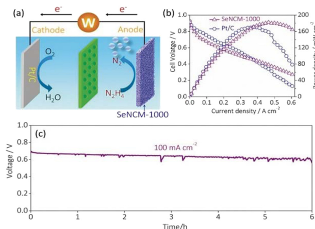
Fig. 26 (a) Schematic diagram of O 2 -HzFC. (b) Polarization and power density plots for O 2 -HzFCs at 80 °C with Se-doped and Pt/C catalysts, respectively. (c) Long-term stability of the O 2 -HzFC with the Se-doped catalyst. Reproduced with permission from ref. 62. © 2019 Wiley-VCH GmbH.
