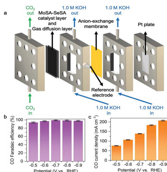
Fig. 27 Performance evaluation of the Mo-Se DASC in a GDE-based flow-cell. (a) Scheme of the GDE-based flow-cell. (b) FE CO of the Mo-Se DASC in the constant potential flow-cell test. (c) j CO in the constant potential flow-cell test. Reproduced with permission from ref. 50. © 2022 Wiley-VCH GmbH.
