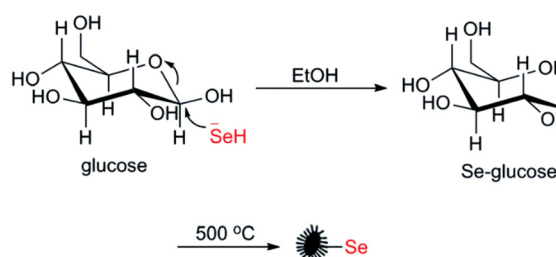
Fig. 15 Fabrication of the Se/C carbonaceous catalysts via glucose selenization and pyrolysis. Adapted with permission from ref. 75. Copyright 2018, The Royal Society of Chemistry.
