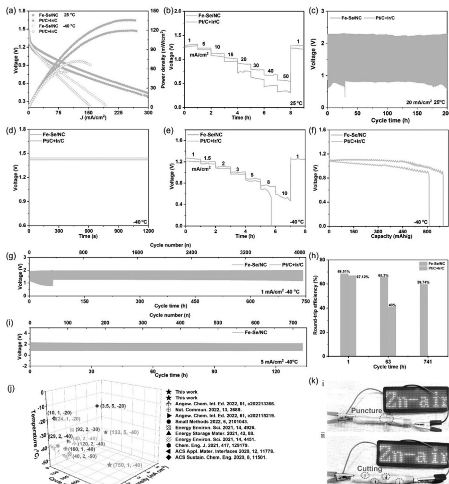
Fig. 23 The electrochemical performance of ZABs–Fe–Se/NC. (a) Discharging polarization curves and the corresponding power density plots at 25 and -40^{\circ}\text{C} . (b) Discharging plateaus with current densities from 1 to 50\text{ mA cm}^{-2} of ZABs–Fe–Se/NC and Pt/C + Ir/C at 25^{\circ}\text{C} . (c) Galvanostatic cycling of ZABs–Fe–Se/NC and ZABs–Pt/C + Ir/C at 20\text{ mA cm}^{-2} at 25^{\circ}\text{C} . (d) OCVs of ZABs–Fe–Se/NC and Pt/C + Ir/C at -40^{\circ}\text{C} . (e) Discharging plateaus with current densities from 1 to 10\text{ mA cm}^{-2} . (f) Capacity, (g) galvanostatic cycling, and (h) the corresponding round-trip efficiency decay of ZABs–Fe–Se/NC and ZABs–Pt/C + Ir/C at 1\text{ mA cm}^{-2} at -40^{\circ}\text{C} . (h) Comparison of the round-trip efficiency decay. (i) Galvanostatic cycling at 5\text{ mA cm}^{-2} of ZABs–Fe–Se/NC at -40^{\circ}\text{C} . (j) Comparison with reported low-temperature ZABs. The values of coordinates ( m, n, o ) in the graph represent the cycle time, current density, and operating temperature, respectively. (k) Optical images of LED screens powered by ZABs–Fe–Se/NC under (i) puncturing and (ii) cutting. Reproduced with permission from ref. 48. © 2023 Wiley-VCH GmbH.
