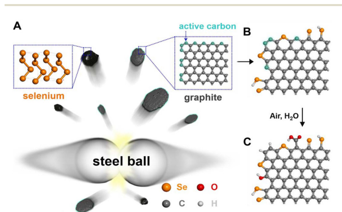
Fig. 12 Schematic representation of ball-milling the mixture of graphite and Se powder to produce edge-selenated graphene nanoplatelets. Reproduced with permission from ref. 66. Copyright © 2016, The Authors.
