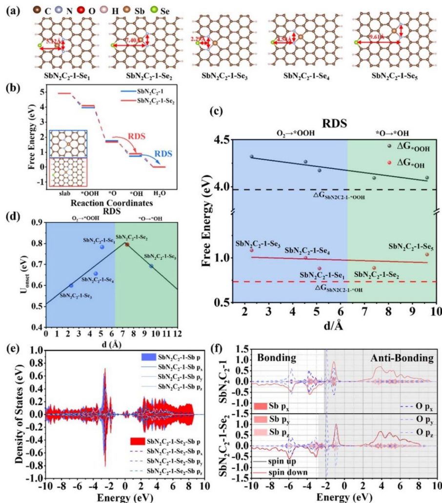
Fig. 24 DFT calculations on the long-range regulation mechanism. (a) The structure diagram and the distance between Se and N of \text{SbN}_2\text{C}_2\text{-1-Se}_n ( n=1-5 ). (b) Free energy diagram of \text{SbN}_2\text{C}_2 and \text{SbN}_2\text{C}_2\text{-1-Se}_2 , RDS represents the rate-determining step. (c) The RDS of different structures and the free energy diagram of intermediates ^*\text{OH} and ^*\text{OOH} . The dotted line represents \Delta G_{\text{SbN}_2\text{C}_2\text{-1}} . The blue and green background represents the RDS of the first three and latter two structures, respectively. (d) The U_{\text{onset}} of \text{SbN}_2\text{C}_2\text{-1-Se}_n ( n=1-5 ). (e) The PDOS of \text{SbN}_2\text{C}_2\text{-1-Sb} and \text{SbN}_2\text{C}_2\text{-1-Se}_2\text{-Sb} . (f) The PDOS of \text{SbN}_2\text{C}_2\text{-1-Sb} and \text{SbN}_2\text{C}_2\text{-1-Se}_2\text{-Sb} . (f) Suborbital PDOS of the O and Se orbitals combined with the bonding state shown by the crystal orbital Hamilton population (COHP); light gray means the density of states is the bond state, and dark gray is the anti-bond state. Reproduced with permission from ref. 51. Copyright © 2023, American Chemical Society.
