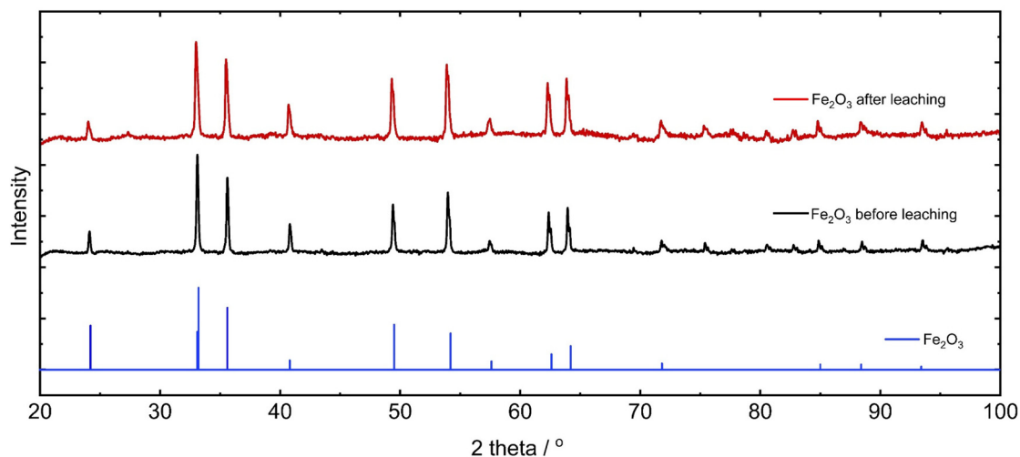
Fig. 2 XRD patterns of Fe 2 O 3 before (black) and after (red) leaching, and \alpha -Fe 2 O 3 standard (JCPDS no. 04-022-0741) (blue).
