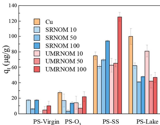
Fig. 3 Adsorption capacity of Cu onto PS-virgin, PS-O 3 , PS-SS and PS-lake in Cu solution with DOM (concentration of DOM: 0, 10, 50, 100 \text{mg L}^{-1} ).
