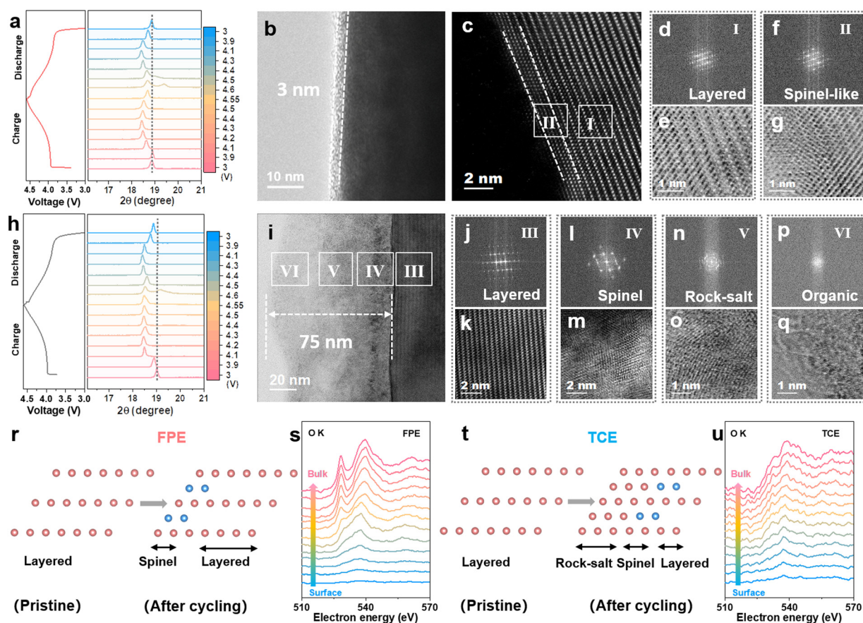
Fig. 4 Characterization of the CEI layer and surface evolution of the 4.6 V LCO cathode during the charge/discharge processes. (a) Selected region of the (003) plane from the ex situ XRD patterns of LCO electrode cycled in FPE during the 4th charging–discharging process at 0.2C. (b) HRTEM and (c) high angle annular dark field scanning transmission electron microscope images of 4.6 V LCO cathode particles after 500 cycles in FPE. (d) The fast Fourier transform (FFT) and (e) inverse fast Fourier transform (IFFT) patterns of selected regions marked (I). (f) The FFT and (g) IFFT patterns of selected regions marked (II). (h) Selected region of the (003) plane from the ex situ XRD patterns of LCO electrode cycled in TCE during the 4th charging–discharging process at 0.2C. (i) HRTEM image of 4.6 V LCO cathode particles after 500 cycles in TCE. (j) The FFT and (k) IFFT patterns of selected regions marked (III). (l) The FFT and (m) IFFT patterns of selected regions marked (IV). (n) The FFT and (o) IFFT patterns of selected regions marked (V). (p) The FFT and (q) IFFT patterns of selected regions marked (VI). (r) Schematic diagram of atomic configuration evolution and (s) EELS spectra of O K-edge from the surface to the inner bulk of the cycled LCO cathodes in FPE. (t) Schematic diagram of atomic configuration evolution and (u) EELS spectra of O K-edge from the surface to the inner bulk of the cycled LCO cathodes in TCE.
