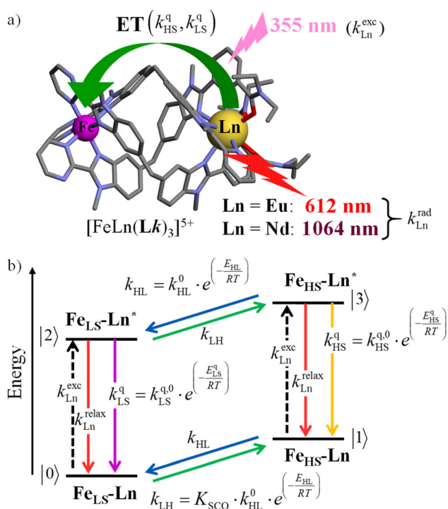
Fig. 8 (a) Fe(II)-modulated light downshifting operating in [\text{Fe(II)Ln(Lk)}_3]^{5+} helicates (ET = energy transfer) and (b) associated four-states kinetic model.
