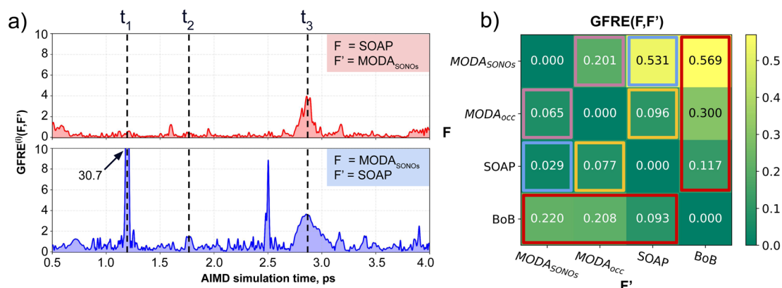
Fig. 6 (a) Point-wise Global Feature Reconstruction Error GFRE^{(t)}(F, F') during the 0.5–4 ps time interval of AIMD. The upper panel (red curve) shows the error spectrum associated to the reconstruction of MODA_{SONOs} ( F' ) using SOAP ( F ), while the lower panel (blue curve) corresponds to the reconstruction of SOAP features ( F' ) using MODA_{SONOs} ( F ). Dashed black lines indicate three different time regions discussed in the main text. The matrix in (b) indicates the Global Feature Reconstruction Error GFRE(F, F') using the descriptors in each row ( F ) to reconstruct the descriptor indicated in each column label ( F' ). Some matrix elements are highlighted to facilitate the discussion in the text (using color frames).
