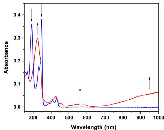
Fig. 9 UV-Vis absorption spectral changes resulting from oxidation of m -ICz-Br (blue) to [ m -ICz-Br] + (red.). Conditions: in CH 2 Cl 2 /Bu 4 NPF 6 at T = 298 K; Pt minigrad in an OTTLE cell.
