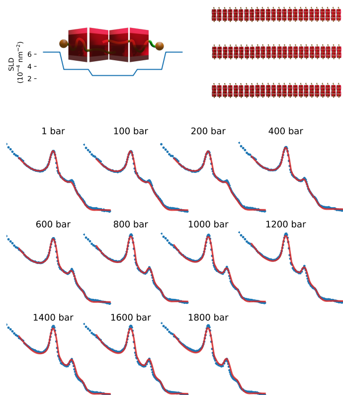
Fig. 2 SANS scattering intensities from \alpha CD- C_{12}E_5CH_2COONa complexes at different hydrostatic pressure values. Solid lines are best fits according to a model of stacked membranes, as described in the text. For absolute intensities and scattering vector values refer to Figure 1.
