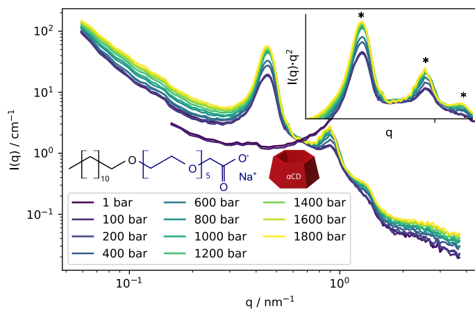
Fig. 1 Small-angle neutron scattering data from a \alpha CD- C_{12}E_5CH_2COOH complexes as a function of the applied hydrostatic pressure. Inset shows region at mid- q with the correlation peaks stemming from the multilayered order within the aggregates in a I(q) \cdot q^2 vs. q representation for improved readability. Peak positions of q^* = [0.45, 0.90, 1.35] nm^{-1} are marked with *
