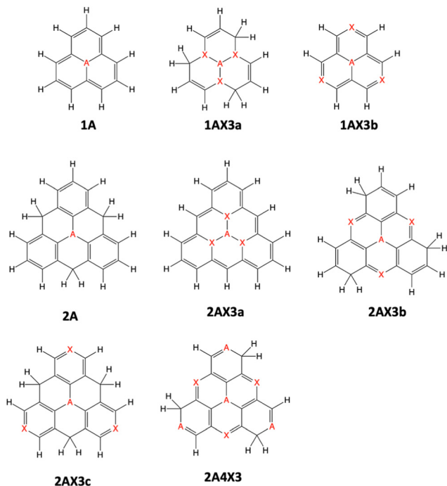
Fig. 1 Studied N and B doped phenalenenes and triangulenes with (A,X) = (B,N) or (A,X) = (N,B).
