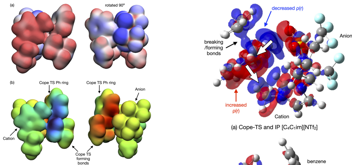
Fig. 13 Reaction B TS-[C 4 C 1 C 1 im][NTf 2 ] (a) electrostatic potential (ESP) mapped onto the 0.007 density iso-surface, red positive, blue negative, maximum \pm 0.05 a.u., (b) \Delta\rho = \rho_{\text{cluster}} - (\rho_{\text{TS}} + \rho_{\text{solvent}}) mapped onto the 0.007 a.u. ( e/a_0^3 ) density iso-surface. "Rainbow" colour scheme, blue = negative, green = neutral, red = positive, maximum \pm 0.02 a.u.
