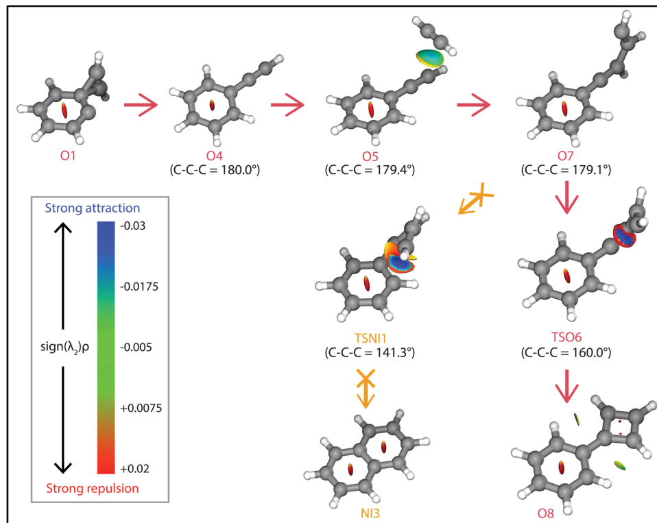
Fig. 8 NCI plots of intermediates and transition states of the reaction pathways towards phenylcyclobutadiene*+ ( O8 , red arrows), and naphthalene*+ ( NI3 , orange arrows). The strengths of the NCIs are shown by the color spectrum ranging from red (strong repulsion), green (weak attraction) and blue (strong attraction). The calculated angle of the C–C–C group is shown next to the structures.
