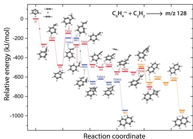
Fig. 7 Potential energy surfaces of the reaction of o -benzyne •+ (O) with acetylene towards the product with m/z 128 phenylcyclobutadiene •+ (O8, red pathway) and naphthalene •+ (N13, purple and orange pathways). The small dots along the pathway display the addition of a new acetylene molecule. The energies are calculated at the B3LYP-GD3/N07D level of theory and are corrected for the zero-point vibrational energy.
