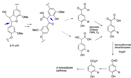
Fig. 5 4-Hydroxybenzoylformate catabolic pathway in R. jostii RHA1, responsible for degradation of aryl C 2 lignin fragments, which may be derived from \beta -5 units in polymeric lignin. 95 R = H or OCH 3 .
