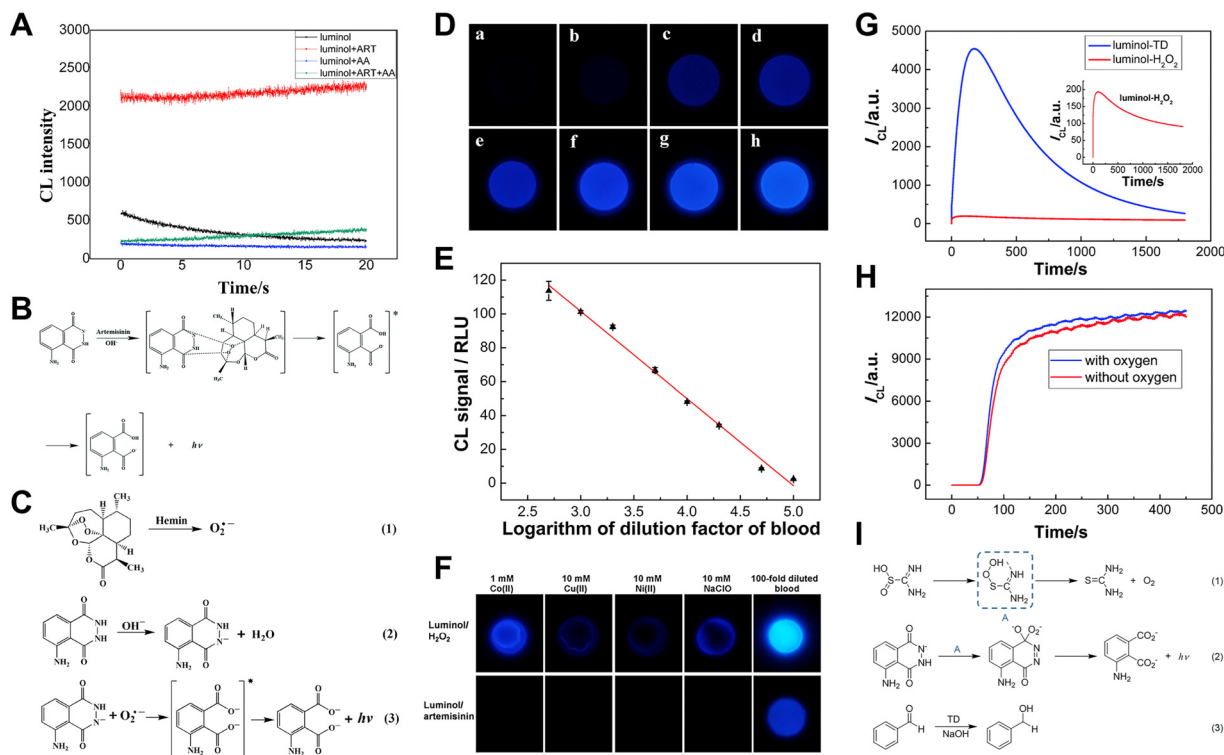
Fig. 1 (A) The CL intensity–time curves of the luminol, luminol/artemisinin, luminol/ascorbic acid (AA) and luminol/artemisinin/AA systems. [Luminol]: 1 mM; [artemisinin]: 4 mM; [AA]: 1 μM; pH: 12.30; PMT voltage: –1100 V. (B) The CL reaction mechanism between luminol and artemisinin. Reprinted with permission from ref. 26, Copyright 2021 Royal Society of Chemistry. (C) The CL mechanism of the luminol/artemisinin/hemin system. (D) CL images of blood samples of different dilution factors: (a) 100 000, (b) 50 000, (c) 20 000, (d) 10 000, (e) 5000, (f) 2000, (g) 1000, and (h) 500. (E) The relationship curve of CL intensities versus the logarithm of the dilution factors of blood. (F) Comparison between luminol/H 2 O 2 and luminol/artemisinin CL systems in distinguishing blood from NaClO and common metal ions Co 2+ , Cu 2+ , and Ni 2+ . [luminol]: 1.0 mM; [H 2 O 2 ]: 1.0 mM; [artemisinin]: 5.0 mM. Reprinted with permission from ref. 27, Copyright 2017 American Chemical Society. (G) The CL intensity–time curves of the luminol/H 2 O 2 and luminol/TD systems, [luminol]: 0.1 mM; [TD]: 1 mM; [H 2 O 2 ]: 1 mM; PMT voltage: –700 V. (H) The effect of dissolved oxygen on the luminol/TD system. [luminol]: 0.1 mM; [TD]: 10 mM; PMT voltage: –700 V. Reprinted with permission from ref. 28, Copyright 2015 Royal Society of Chemistry. (I) The proposed CL mechanism for the luminol/TD system. Reprinted with permission from ref. 29, Copyright 2022 Royal Society of Chemistry.
