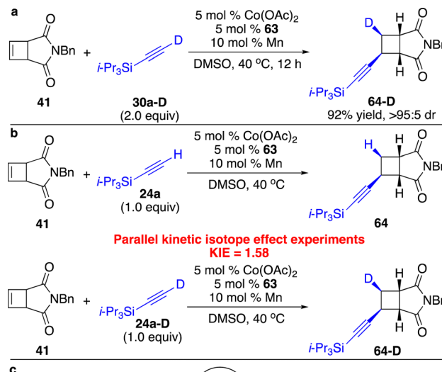
Scheme 21 Mechanistic studies and proposed catalytic cycle for Co-catalyzed enantioselective hydroalkynylation of cyclobutenes. (a) Reaction with deuterated alkyne. (b) Parallel kinetic isotope effect experiments. (c) The proposed catalytic cycle.
