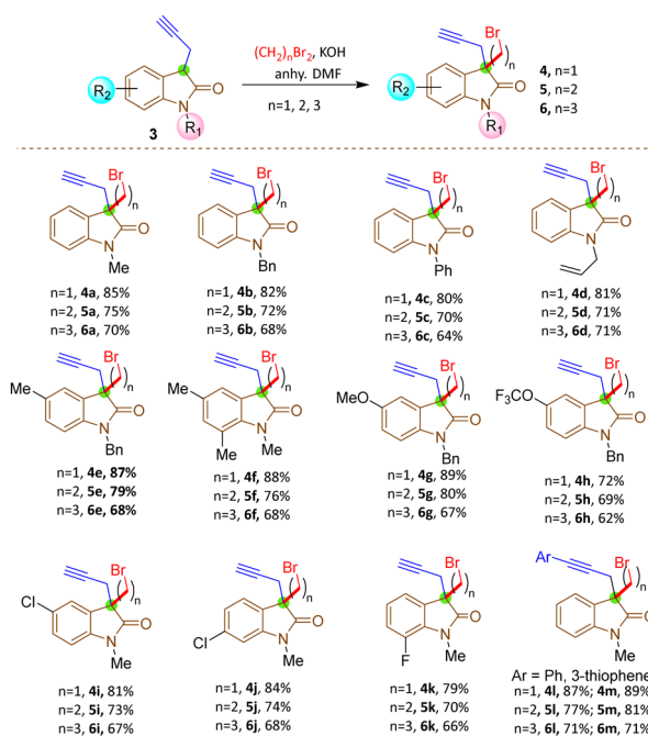
Scheme 2 Synthesis of 3-propargyl substituted oxindoles from isatins. Reaction conditions: (i) 1 (2 mmol), propargyl bromide (6 mmol), Zn dust (12 mmol), \text{HfCl}_4 (0.4 mmol), THF/aq. \text{NH}_4\text{Cl} (1:5, 20 mL) at 0 °C; (ii) 2 (1 mmol), \text{SOCl}_2 (1.2 mmol), DIPEA (3 mmol) in DCM (10 mL) at 0 °C-rt; (iii) Zn dust (6 mmol), AcOH (3 mL) in THF (10 mL) at 0 °C.
