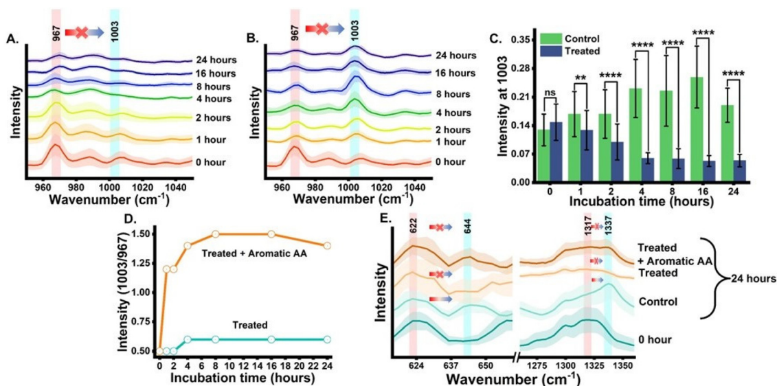
Fig. 3 Validating the peak from the nascent aromatic amino acid in E. coli . (A) Time-dependent mean Raman spectra with standard deviation of E. coli treated with glyphosate. (B) Time-dependent plot mean Raman spectra with standard deviation of glyphosate-treated E. coli supplemented with exogenous aromatic amino acid. (C) Intensity bar plot at 1003 \text{cm}^{-1} of control versus the treated group showing statistical significance (ns ( p > 0.05 ), * ( p \leq 0.05 ), ** ( p \leq 0.01 ), *** ( p \leq 0.001 ), and **** ( p \leq 0.0001 )). (D) Intensity line plot at 1003 \text{cm}^{-1} of the glyphosate-treated group vs. the aromatic amino acid-supplemented glyphosate-treated group. (E) Mean Raman spectra at 0 h and 24 h showing the blue shift of tyrosine and tryptophan peaks under different treatment conditions.
