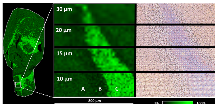
Fig. 3 AgLDI MSI (Ag 6 nm) analysis of cholesterol ( m/z 493.2, [M + 107 Ag] + ). The whole brain section (left) at a spatial resolution of 50 \mu m. The mouse cerebellum (middle) at spatial resolutions of 30 \mu m, 20 \mu m, 15 \mu m, and 10 \mu m illustrates the distinct variations in cholesterol intensity between (A) the lobule/molecular layer, (B) the lobule/granular layer, and (C) fiber tracks. An optical microscope image (right) of the mouse cerebellum shows the section after analysis with laser ablation spots.
