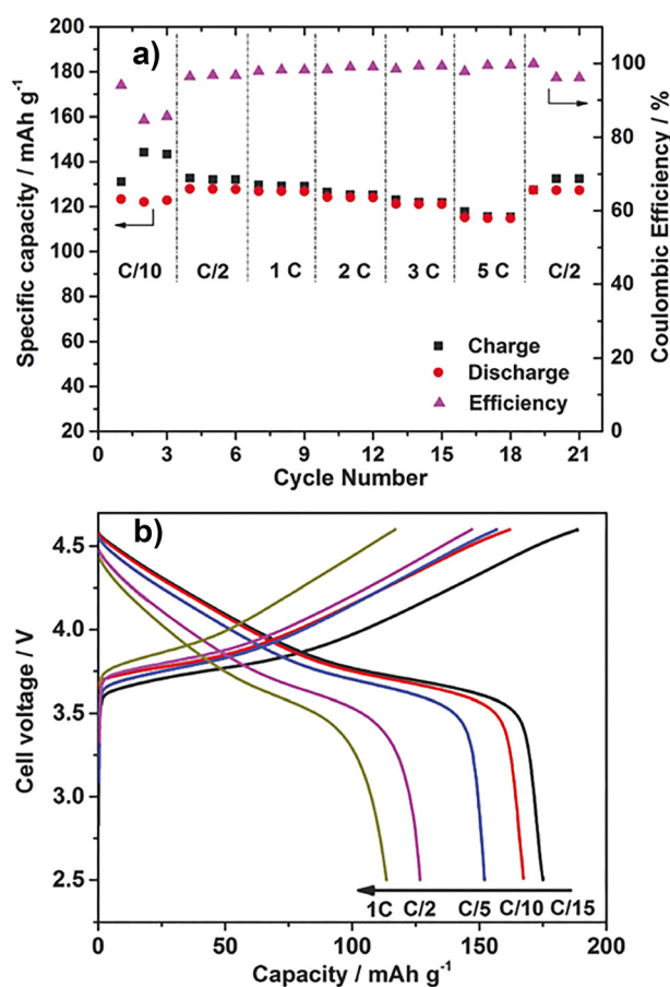
Fig. 10 Electrochemical measurements of 40 wt% \text{Li}_{0.1}\text{Li}_{0.9}\text{b}/\text{PVDF} composites. (a) Specific capacities and coulombic efficiencies of \text{Li}/\text{LiFePO}_4 cells at different current rates, ranging from C/10 to 5C, 50 ^{\circ}\text{C} . (b) Charge-discharge curves of the \text{Li}/\text{LiCo}_{1/3}\text{Ni}_{1/3}\text{Mn}_{1/3}\text{O}_2 cell using 40 wt% \text{Li}_{0.1}\text{Li}_{0.9}\text{b}/\text{PVDF} composites (cut-off voltage 2.5–4.6 V), 50 ^{\circ}\text{C} . (Figure partly modified from the original one.) Reprinted from ref. 94 with permission.
