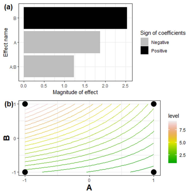
Fig. 4 (a) Pareto plots from the parameters calculated by the mathematical model for Y_2 (adsorption capacity of the composite, mg g -1 ); (b) contour plot of actual values for dosage ( A , g L -1 ) and [ 133 Cs] 0 ( B , mg L -1 ). Levels are predictions for Y_2 (mg g -1 ).
