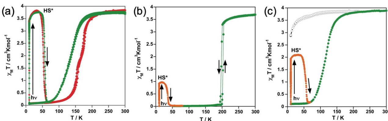
Fig. 1 Magnetic and photomagnetic properties for (a) 1 and 1\cdot\text{CH}_3\text{CN} (red and green solid circles, respectively); (b) 2 (green solid circles) and (c) 3\cdot 1/2\text{CH}_2\text{Cl}_2 (green solid circles) and 3 (black open circles).
