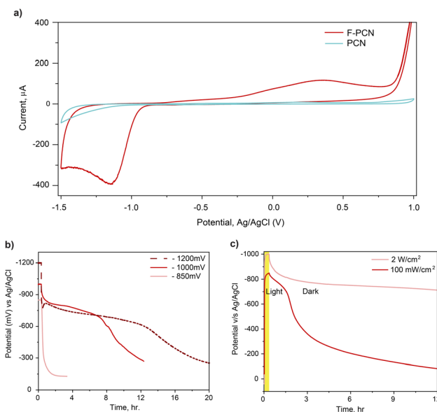
Fig. 2 (a) Cyclic voltammety curve for PCN and F-PCN in 0.1 M \text{Na}_2\text{SO}_4 and 5 mM 4-MBA, scan rate 5 \text{ mV s}^{-1} (b) charging F-PCN for 20 min with three different external biases in \text{Na}_2\text{SO}_4 and 4-MBA electrolyte (c) charging F-PCN in \text{Na}_2\text{SO}_4 and 4-MBA with different intensity lamp (1.5 AM). All the measurements are done under inert conditions.
