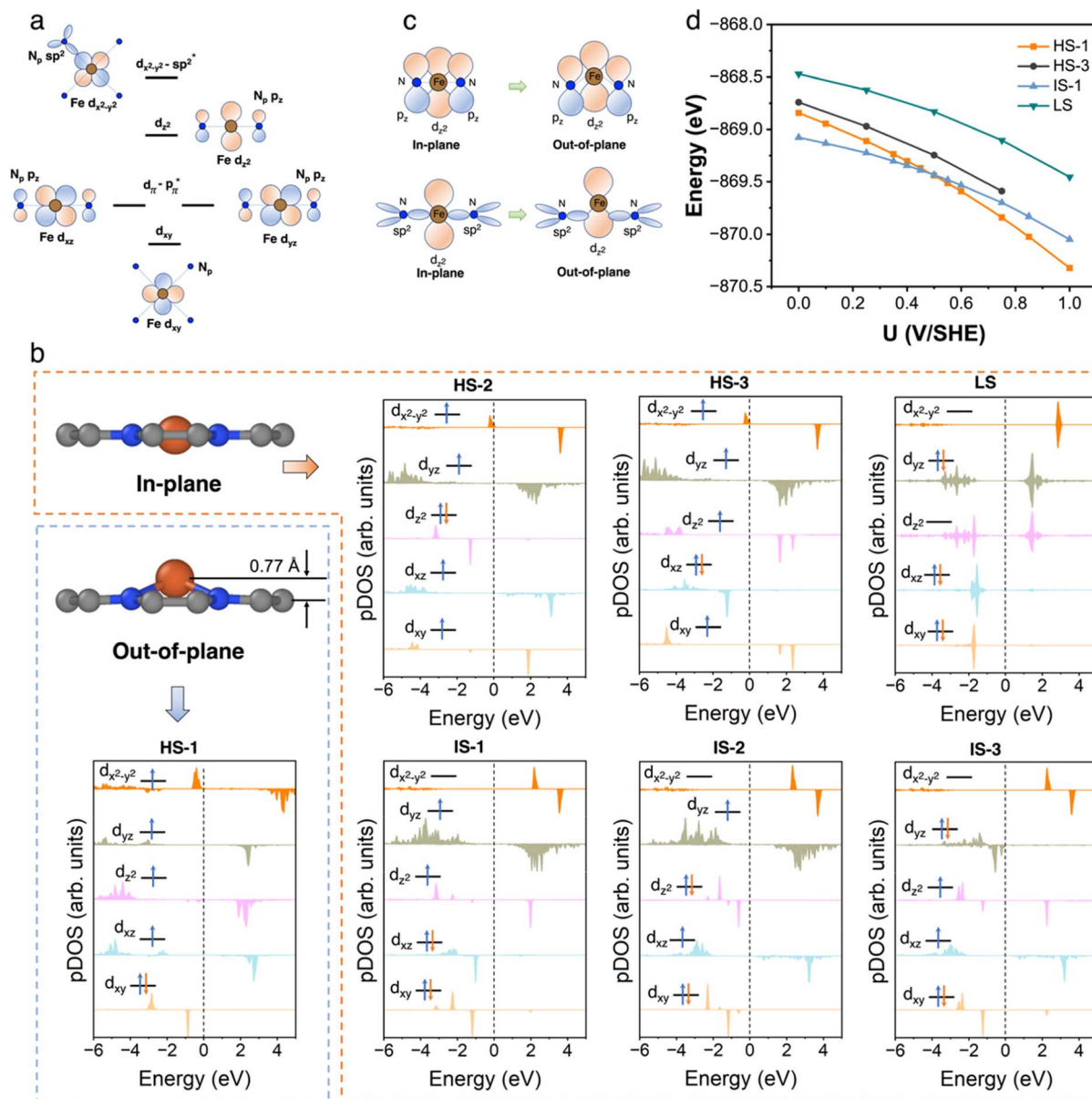
Fig. 2 FeN_4C_{10} . (a) Schematics of the interactions of Fe d orbitals with the orbitals in pyridinic N ( N_p ) in a square-planar ligand field. (b) Atomic structures and pDOS plots of seven stable spin states of bare FeN_4C_{10} . (c) Schematic plots of additional bonding interactions between the Fe d_{z^2} orbital and N p_z or sp^2 orbitals when Fe transforms from an in-plane structure to an out-of-plane structure in FeN_4C_{10} . (d) Potential-dependent energies of FeN_4C_{10} with different spin states under constant-potential conditions.
