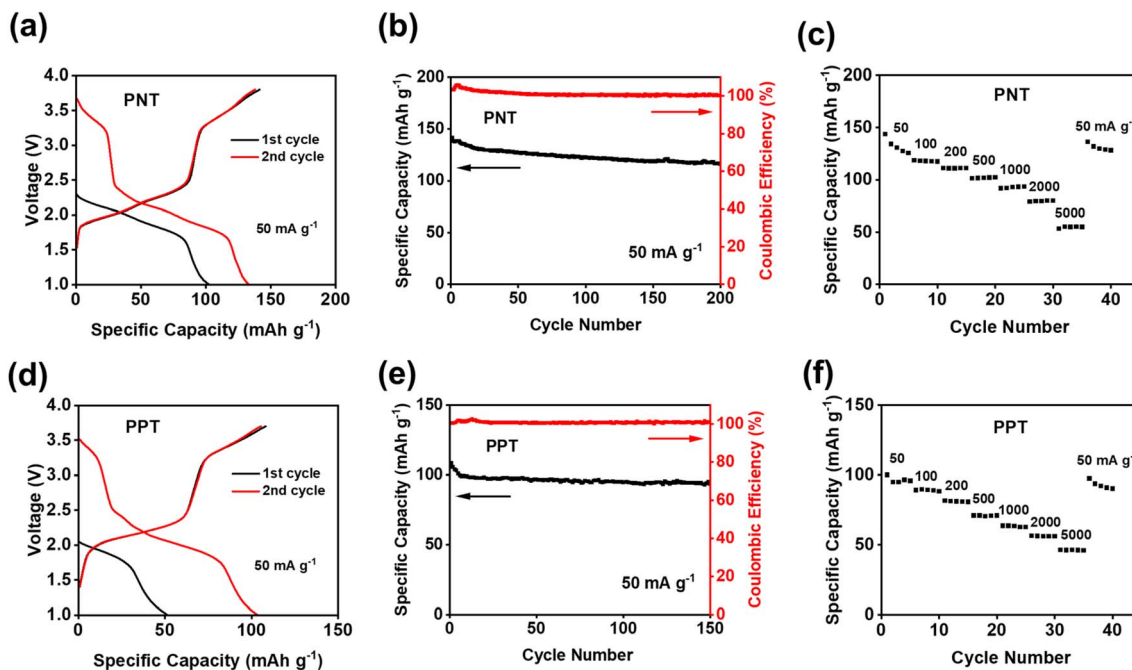
Fig. 3 Electrochemical performance of PNT/PPT with single-layer graphene in NIBs: (a) and (d) galvanostatic charge–discharge curves; (b) and (e) cycling performance; (c) and (f) rate capability at various current densities.
