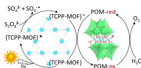
Scheme 5 Proposed mechanism for the light-driven water oxidation by Porp– \text{Co}_4 @MOF-545. Reprinted from ref. 84 with permission from American Chemical Society (Copyright 2018).
