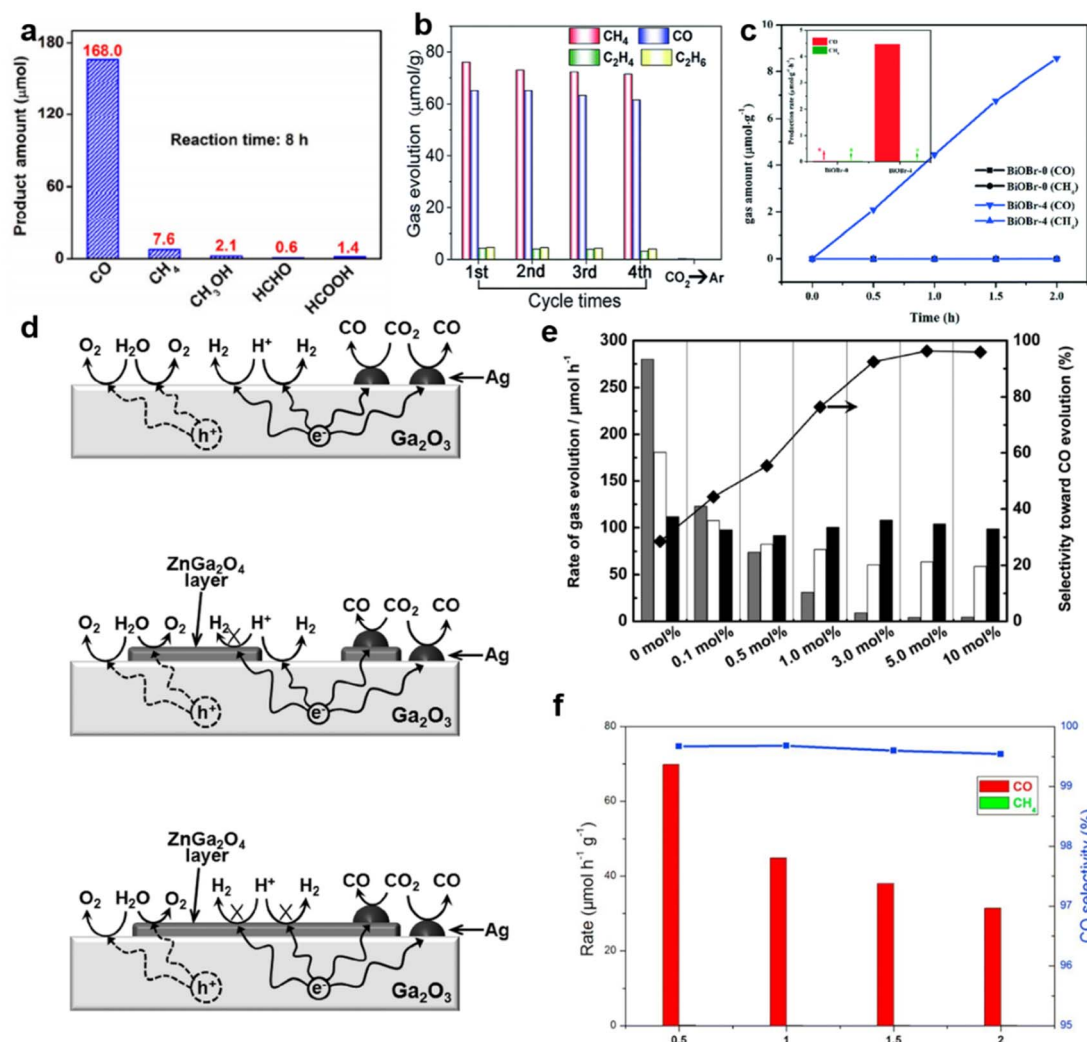
Fig. 3 (a) The amount of products over V_{O_2} -enriched Pt– Ga_2O_3 after irradiation for 8 h. Reproduced with permission from ref. 81 copyright 2018 Springer. (b) Photocatalytic yield and stability of Au–Pd-alloy-decorated TiO_2 . Reproduced with permission from ref. 73. copyright 2019 Royal Society of Chemistry. (c) Production rates of CH_4 and CO over BiOBr photocatalysts under Xe light irradiation. Reproduced with permission from ref. 83 copyright 2017 Royal Society of Chemistry. (d) A proposed mechanism for the photocatalytic conversion of CO_2 in H_2O over Ag-loaded Ga_2O_3 , Ag-loaded Zn-modified Ga_2O_3 with a low Zn content, and Ag-loaded Zn-modified Ga_2O_3 with a high Zn content. (e) Evolution rates of CO (black), O_2 (white), and H_2 (gray) in the photocatalytic conversion of CO_2 over Ag-loaded ZnGa_2O_4 -modified Ga_2O_3 containing different amounts of ZnGa_2O_4 . Reproduced with permission from ref. 67. Copyright 2016 Royal Society of Chemistry. (f) Evolution rates and selectivity over Bi_4O_5Br_2 and Bi_4O_5Br_2 -UN under UV-vis illumination. Reproduced with permission from ref. 72. Copyright 2017 Elsevier.
