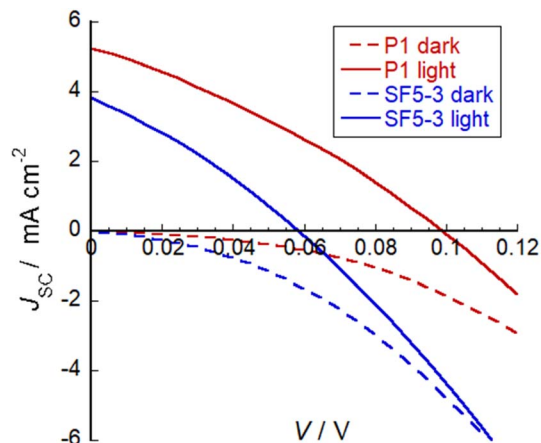
Fig. 7 Plot of current density against voltage for illuminated devices containing dye SF5-3 and the benchmark dye P1. Electrolyte composition: 0.1 M Lil and 1 M I 2 in MeCN.
